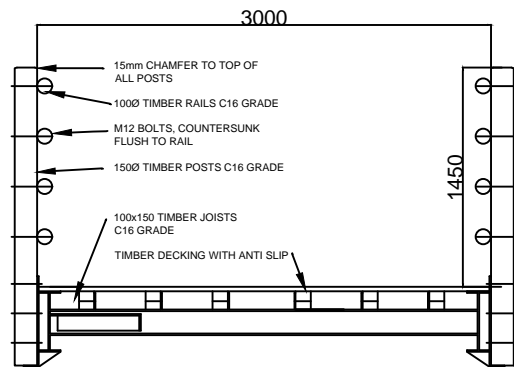
TYPICAL SECTION
