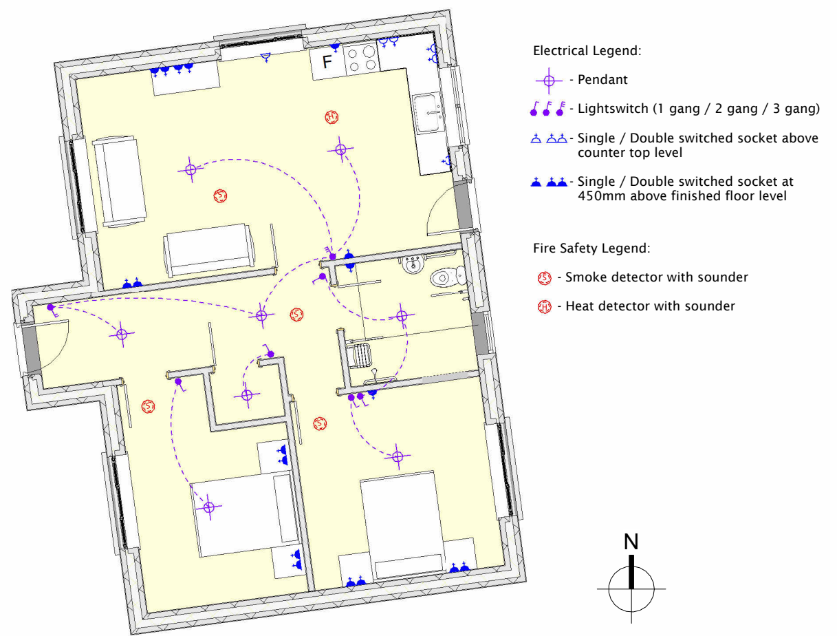
3 Electrical Floor Plan 1 : 100
