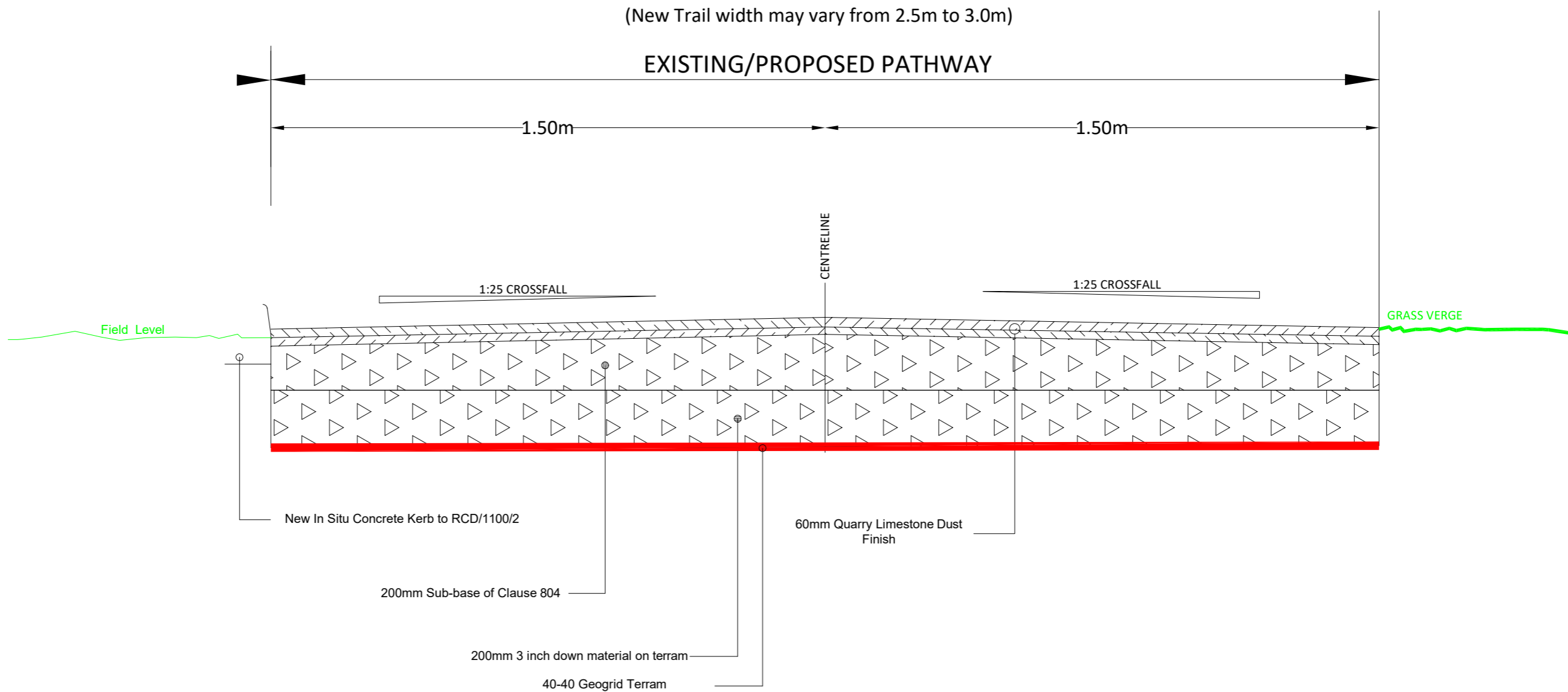
Typical Cross Section A-A
